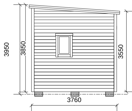
GAVEL LOFT/WC
